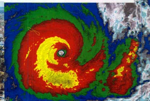
Severe Tropical Cyclone ULUI - 14 March 2010
