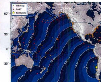
Tsunami Travel Times
